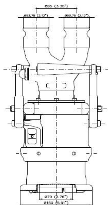
Male Coupling
